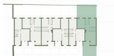
PIANO TERRA
